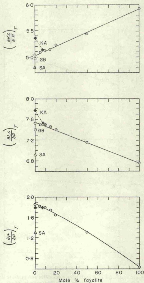
FIG. 3. Pressure derivatives of compressional modulus K_s , shear modulus \mu , and the adiabatic bulk modulus K_s of olivine as a function of (Fe/Mg) ratio; comparison with literature data. ( \Delta ) indicates the datum of Schreiber & Anderson (SA, 1967), ( \square ) indicates the datum of Graham & Barsch (GB, 1969), and ( \diamond ) indicates the data points of Kumasawa & Anderson (KA, 1969); ( \circ ) are the present work.
